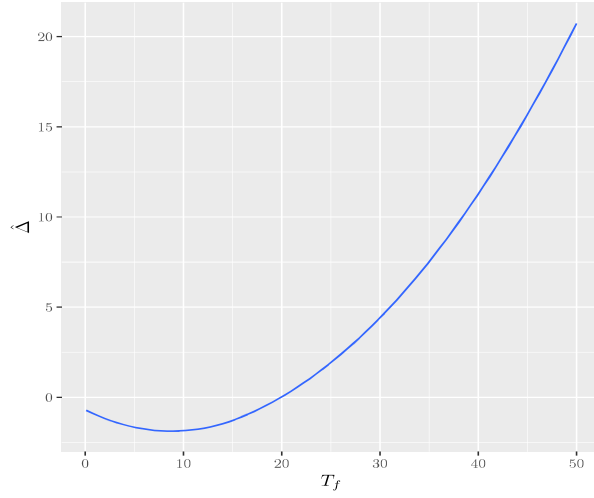
Figure 1: The relation between the size of merging parties and the size of technological synergies required for a merger to be CS-increasing.
