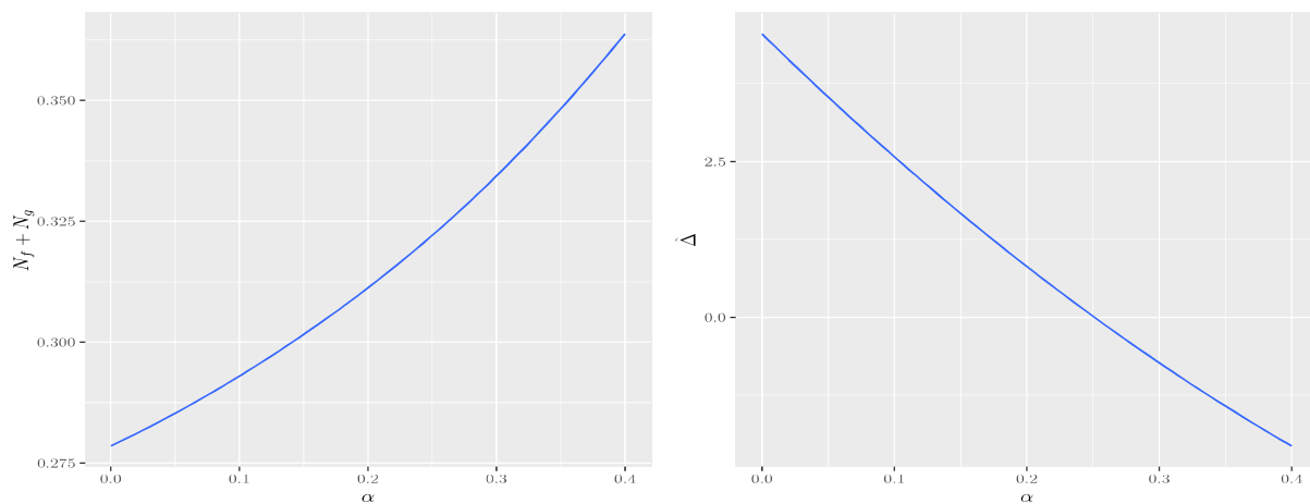
(b) Strong and weak firms ( T_f = 25, T_g = 5 )
