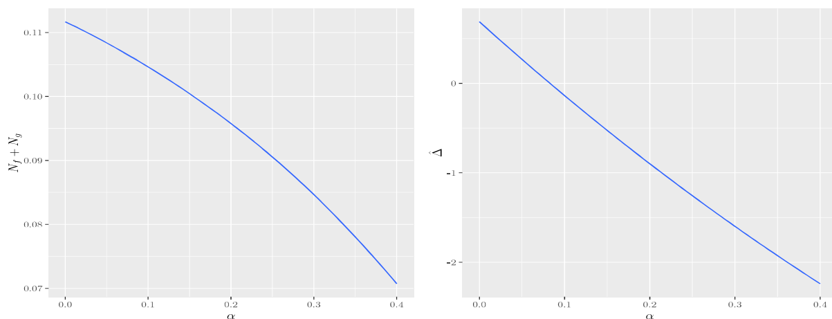
(a) Weak firms ( T_f = T_g = 5 )
