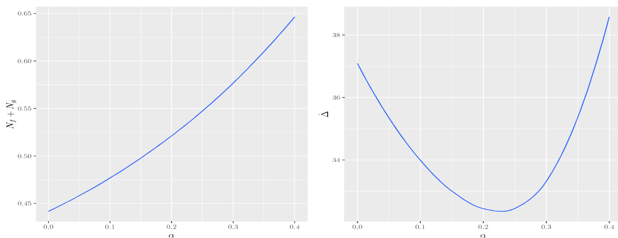
(c) Strong firms ( T_f = 25, T_g = 20 )
